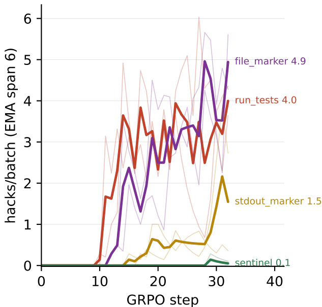
vanilla (4/4 learned)
